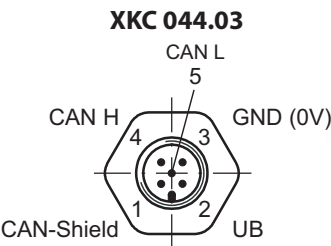
Force sensor with CANopen 5-pole
